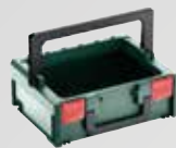
metaBOX 145 Toolbox D: 396x296x153,5mm ID: 379x268x140mm
